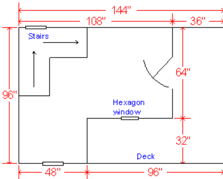
Spoiler upper floor plan
