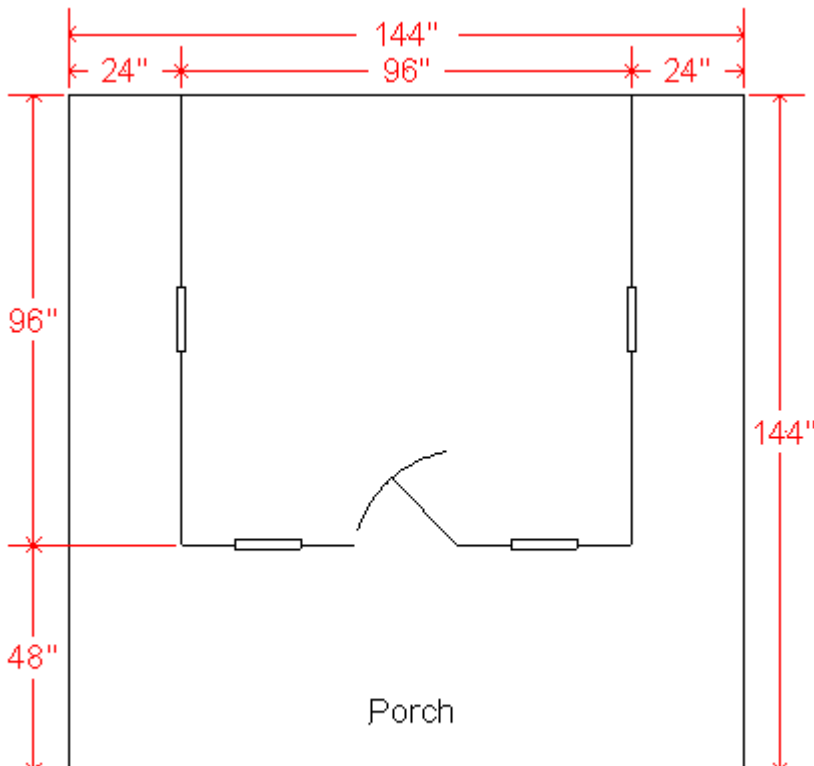
Club House floor plan
