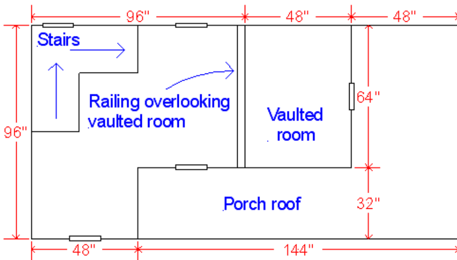
Heritage upper floor plan
