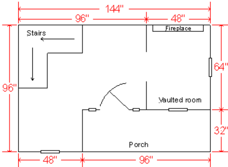
Cottage lower floor plan
