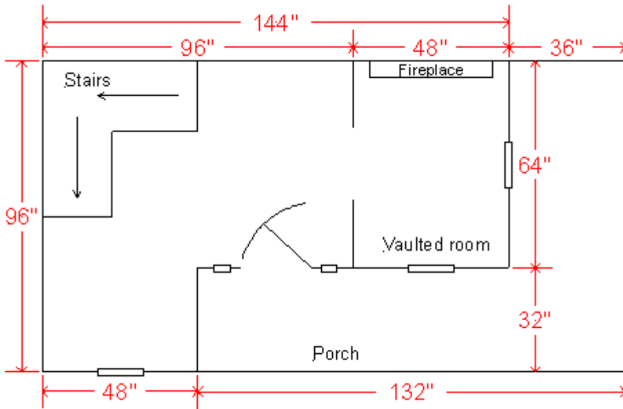
Country Cottage lower floor plan
