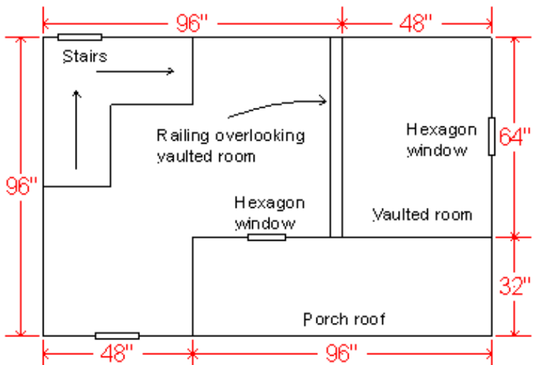
Cottage upper floor plan
