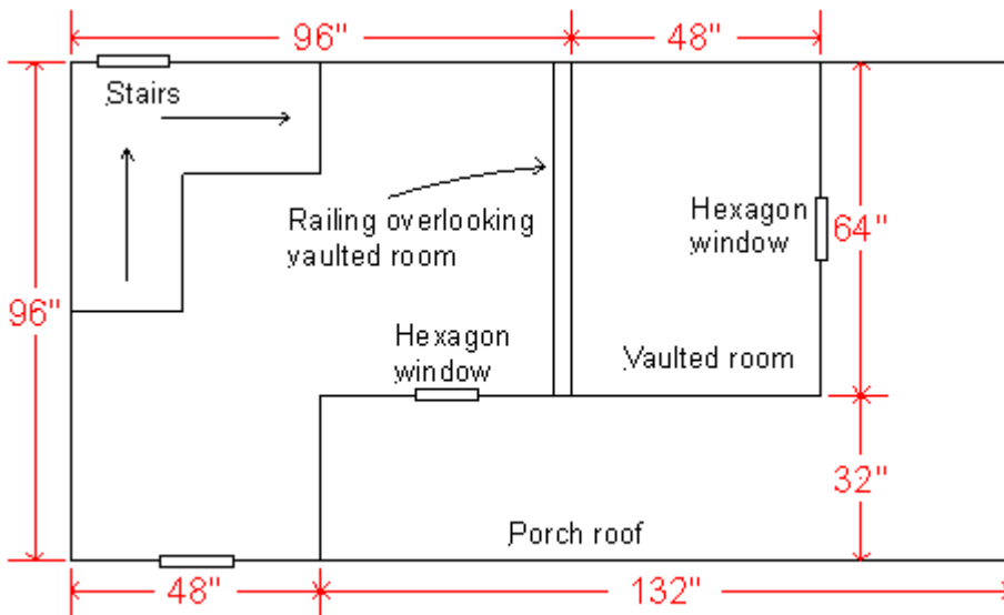
Country Cottage upper floor plan
